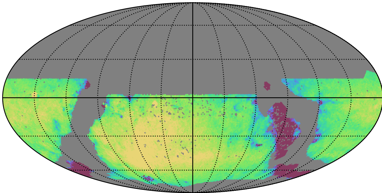
too_10_4v3.4_10yrs WFD g band: Exgal_CoaddM5
