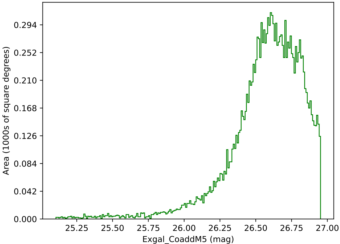
too_10_4v3.4_10yrs WFD g band: Exgal_CoaddM5
