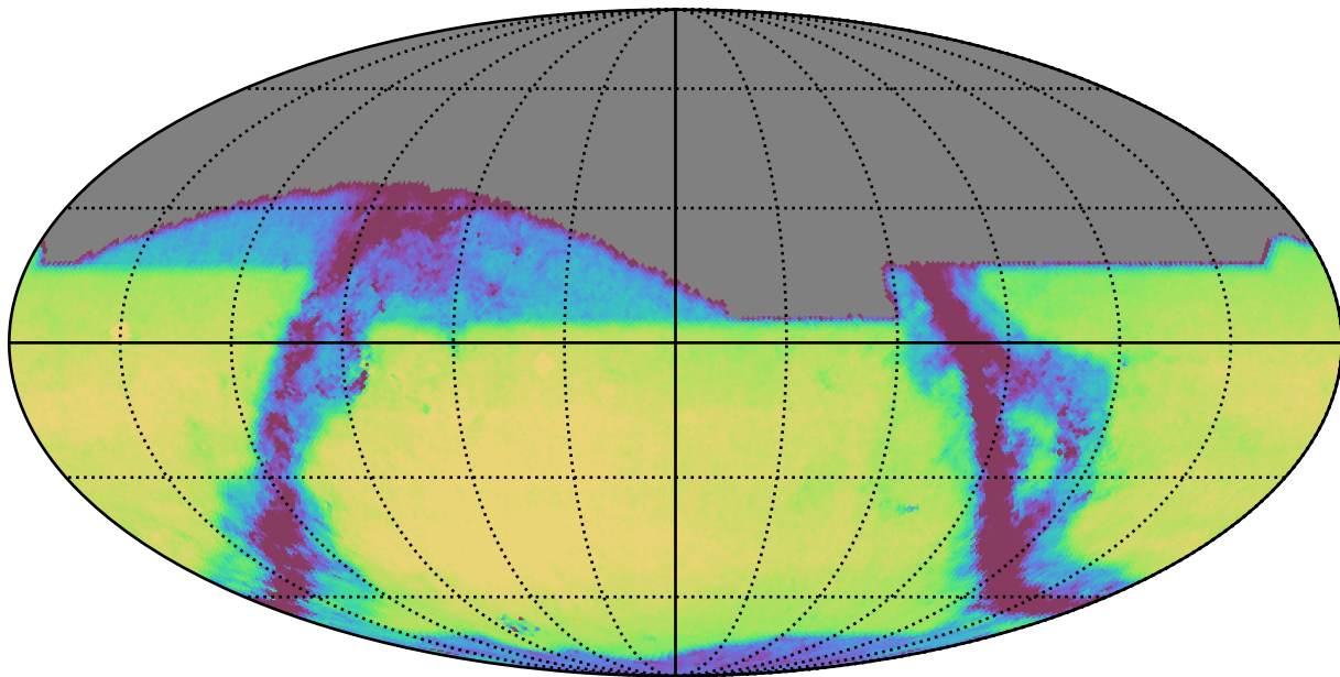
too_10_4v3.4_10yrs All sky z band: Exgal_CoaddM5
