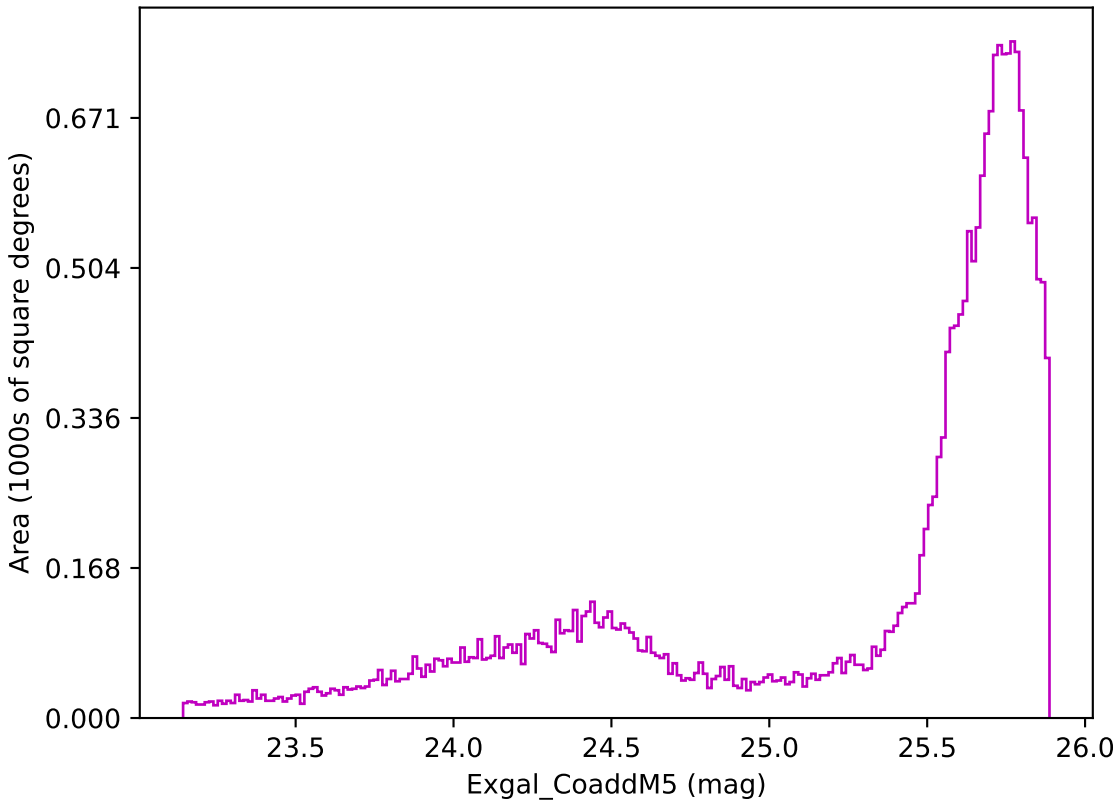
too_10_4v3.4_10yrs All sky z band: Exgal_CoaddM5
