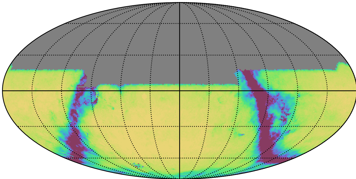
too_10_4v3.4_10yrs All sky u band: Exgal_CoaddM5
