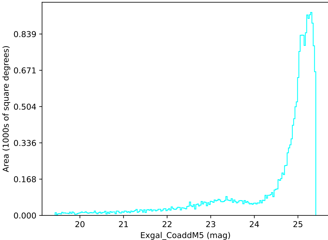
too_10_4v3.4_10yrs All sky u band: Exgal_CoaddM5
