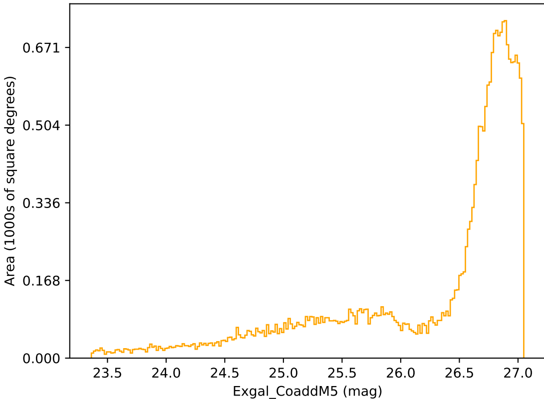
too_10_4v3.4_10yrs All sky r band: Exgal_CoaddM5
