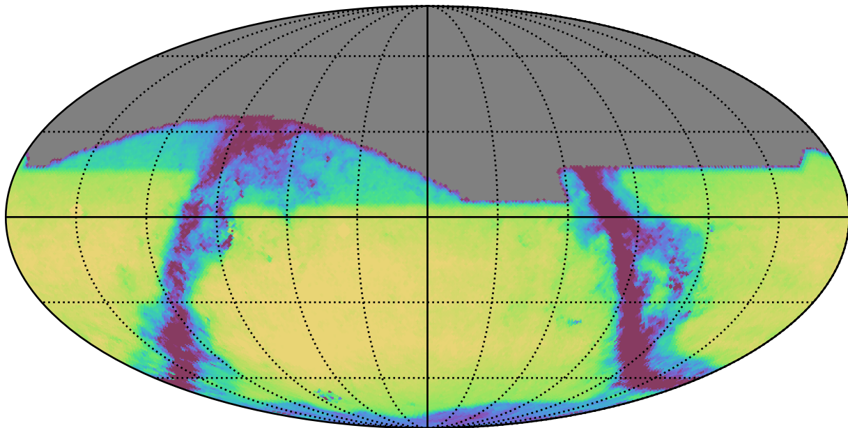
too_10_4v3.4_10yrs All sky i band: Exgal_CoaddM5
