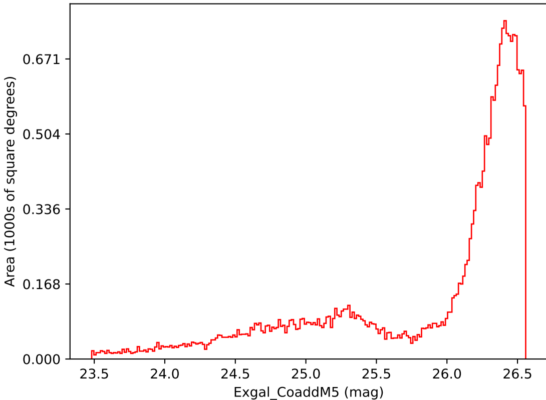
too_10_4v3.4_10yrs All sky i band: Exgal_CoaddM5
