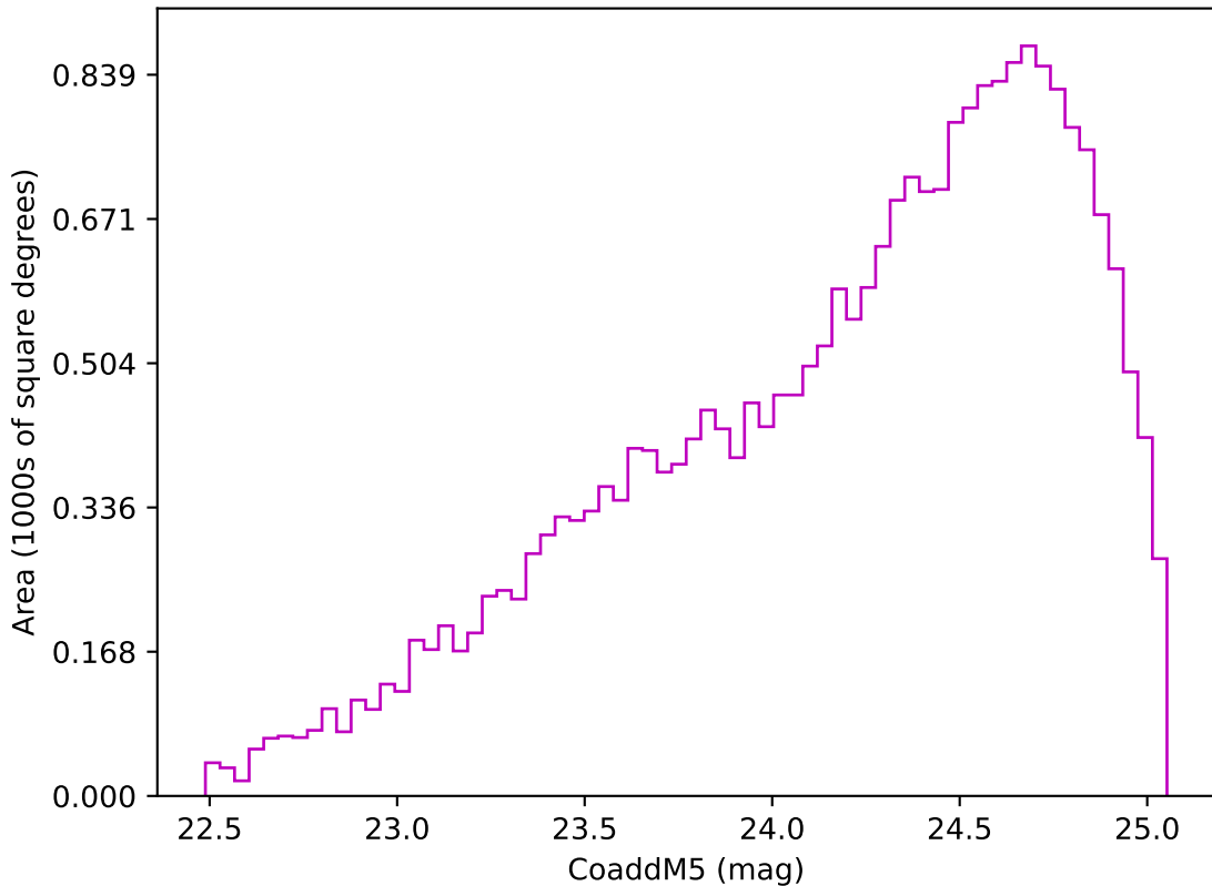
too_10_4v3.4_10yrs Yr 3-4 z band: CoaddM5
