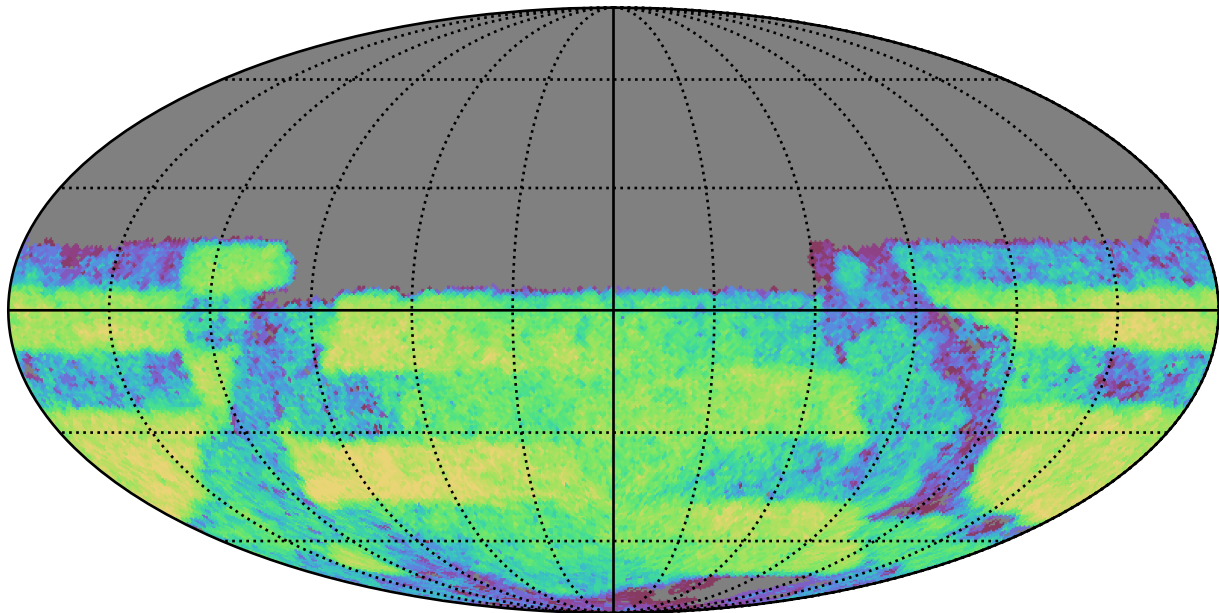
too_10_4v3.4_10yrs Yr 3-4 y band: CoaddM5
