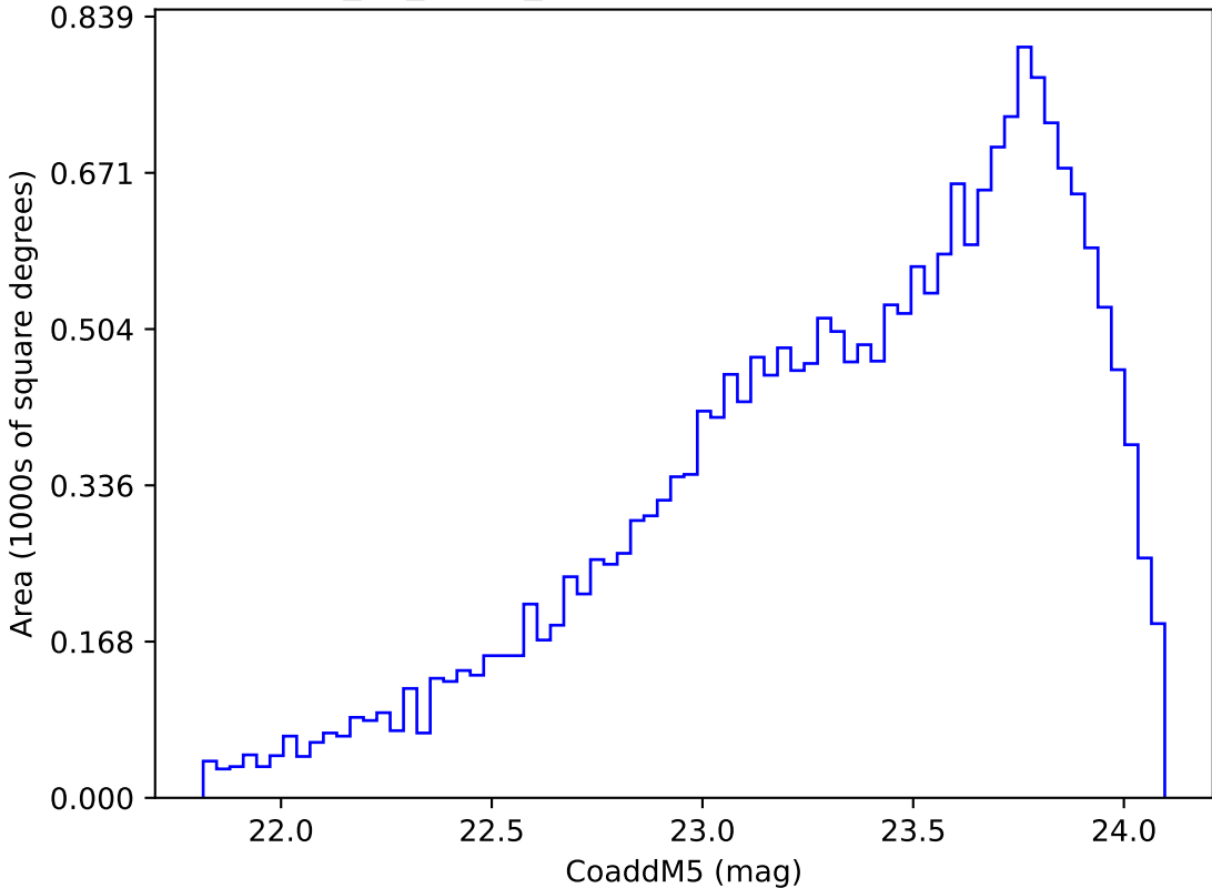
too_10_4v3.4_10yrs Yr 3-4 y band: CoaddM5
