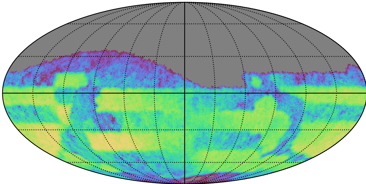
too_10_4v3.4_10yrs Yr 3-4 r band: CoaddM5
