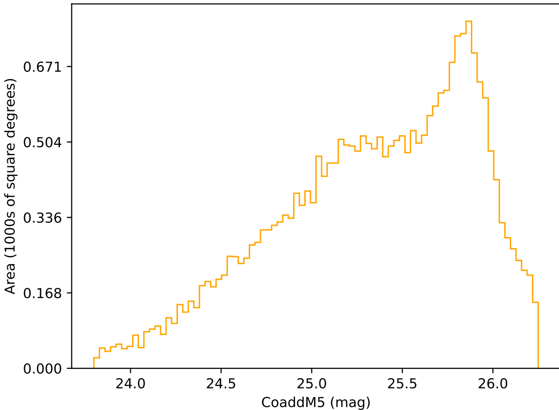
too_10_4v3.4_10yrs Yr 3-4 r band: CoaddM5
