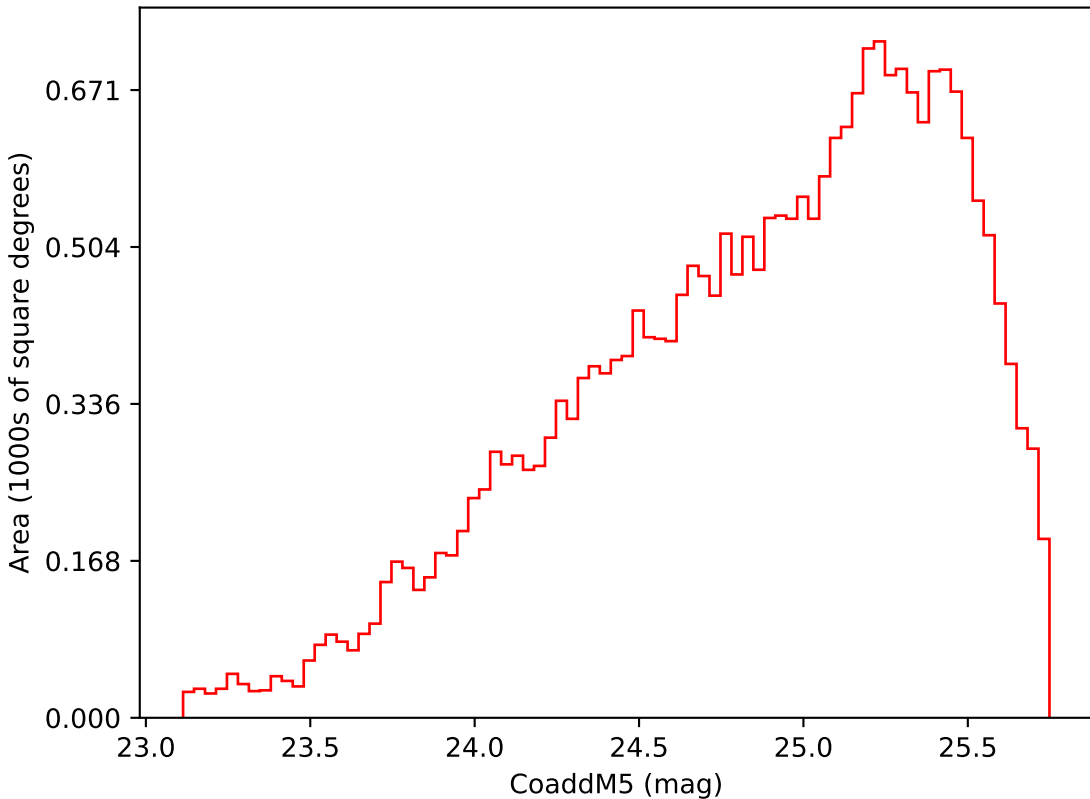
too_10_4v3.4_10yrs Yr 3-4 i band: CoaddM5
