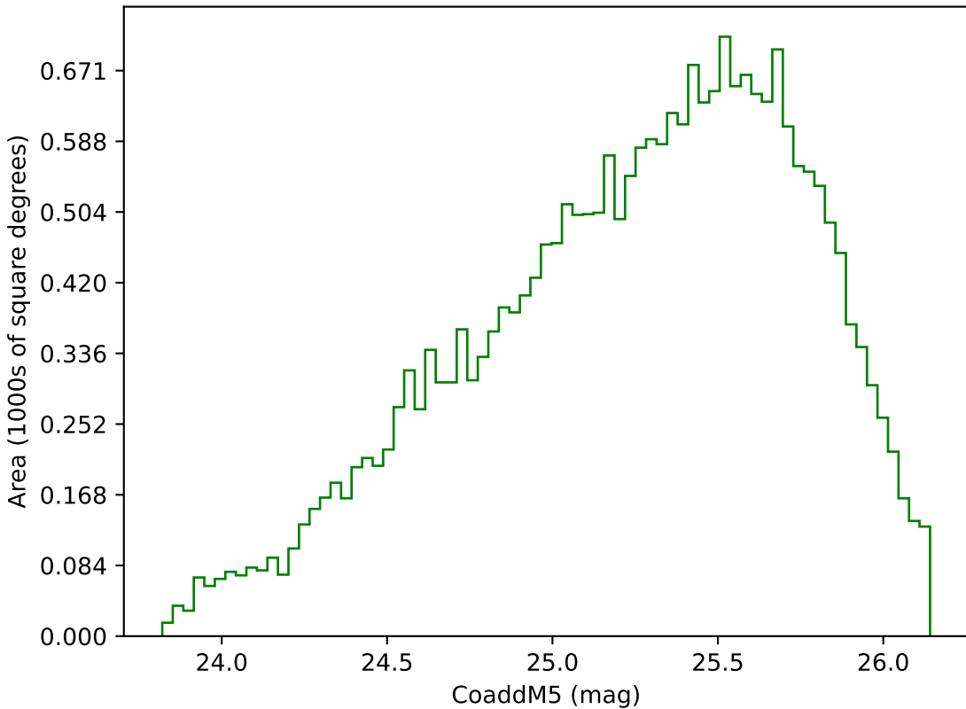
too_10_4v3.4_10yrs Yr 3-4 g band: CoaddM5
