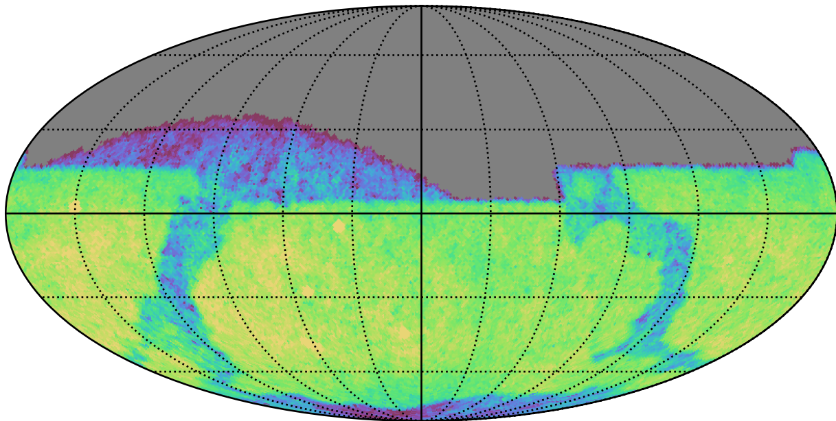
too_10_4v3.4_10yrs Yr 1 z band: CoaddM5
