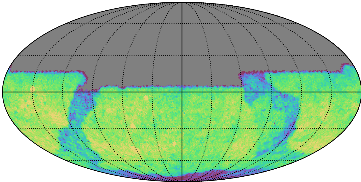
too_10_4v3.4_10yrs Yr 1 y band: CoaddM5
