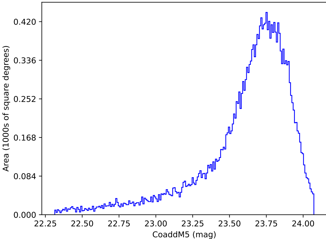
too_10_4v3.4_10yrs Yr 1 y band: CoaddM5
