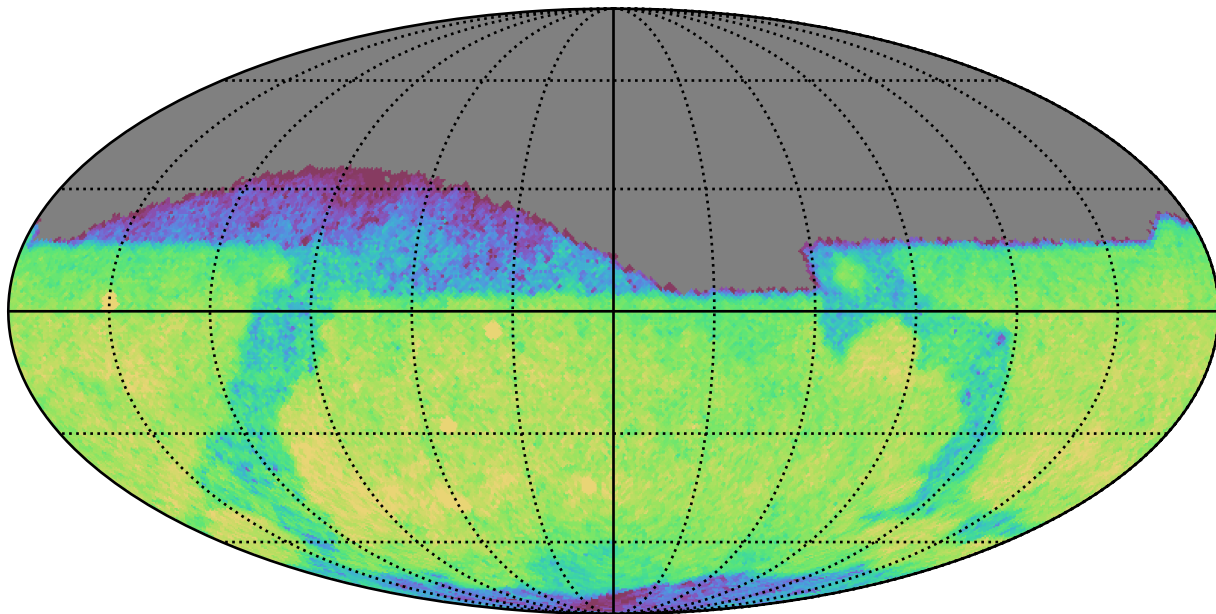
too_10_4v3.4_10yrs Yr 1 r band: CoaddM5
