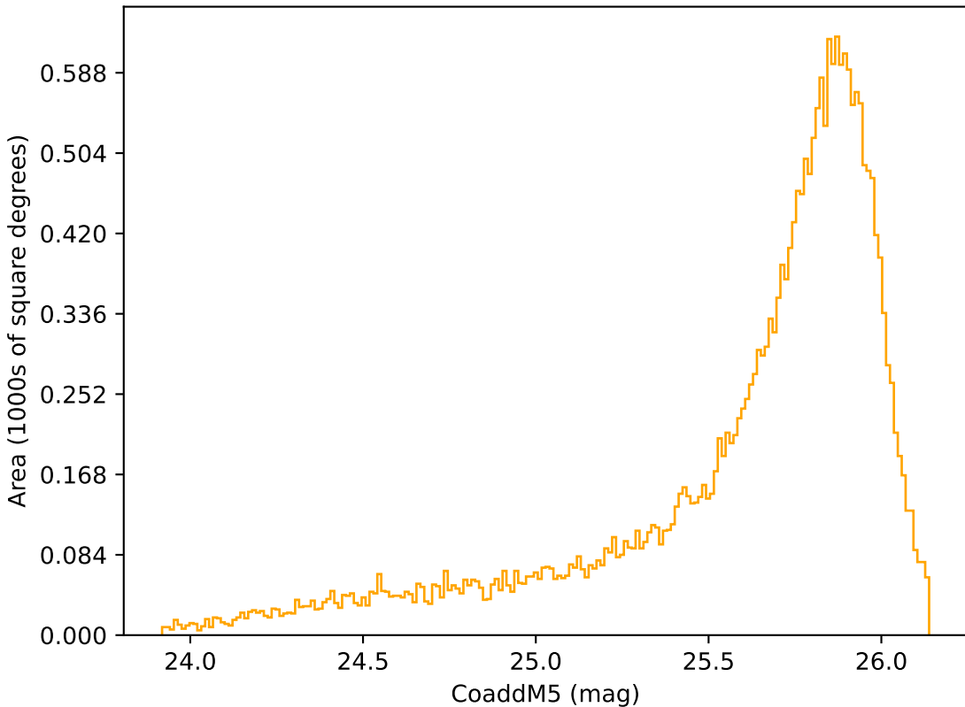
too_10_4v3.4_10yrs Yr 1 r band: CoaddM5
