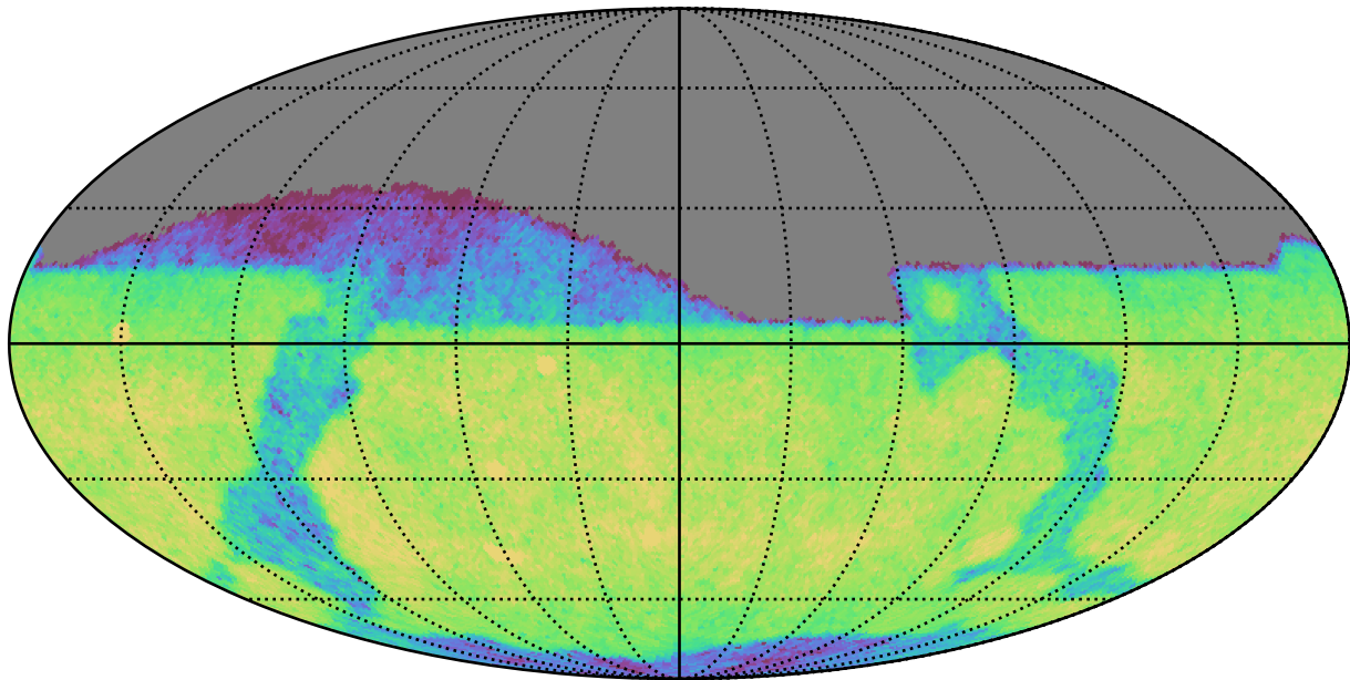
too_10_4v3.4_10yrs Yr 1 i band: CoaddM5
