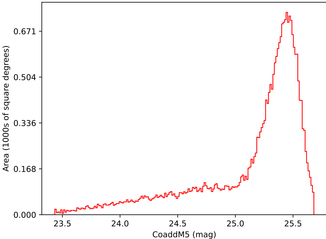
too_10_4v3.4_10yrs Yr 1 i band: CoaddM5
