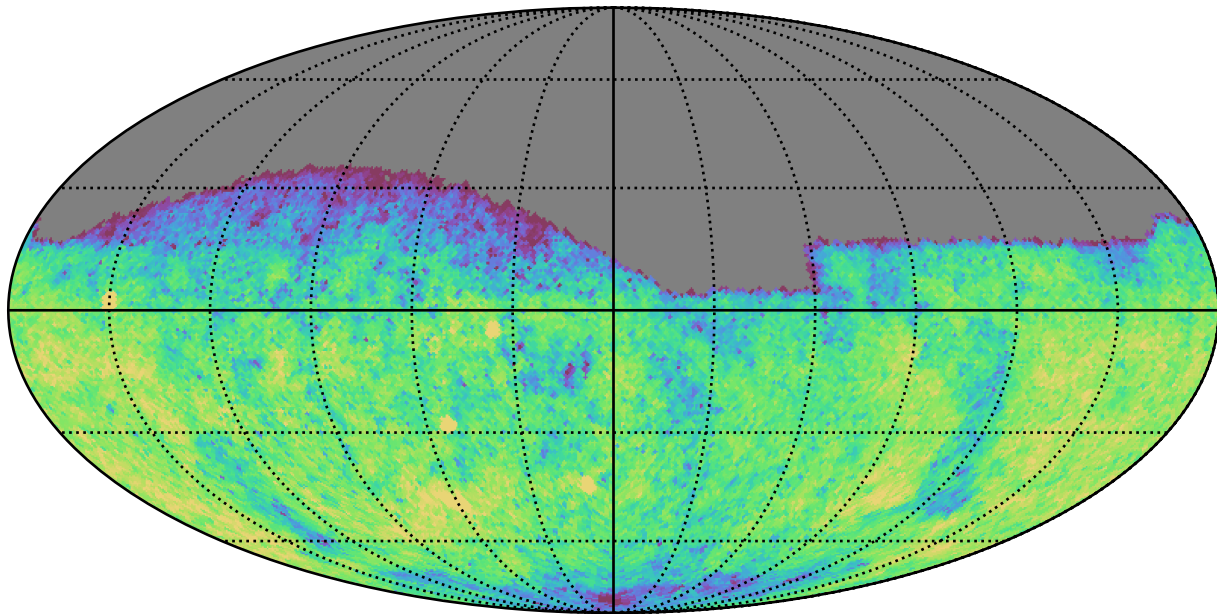
too_10_4v3.4_10yrs Yr 1 g band: CoaddM5
