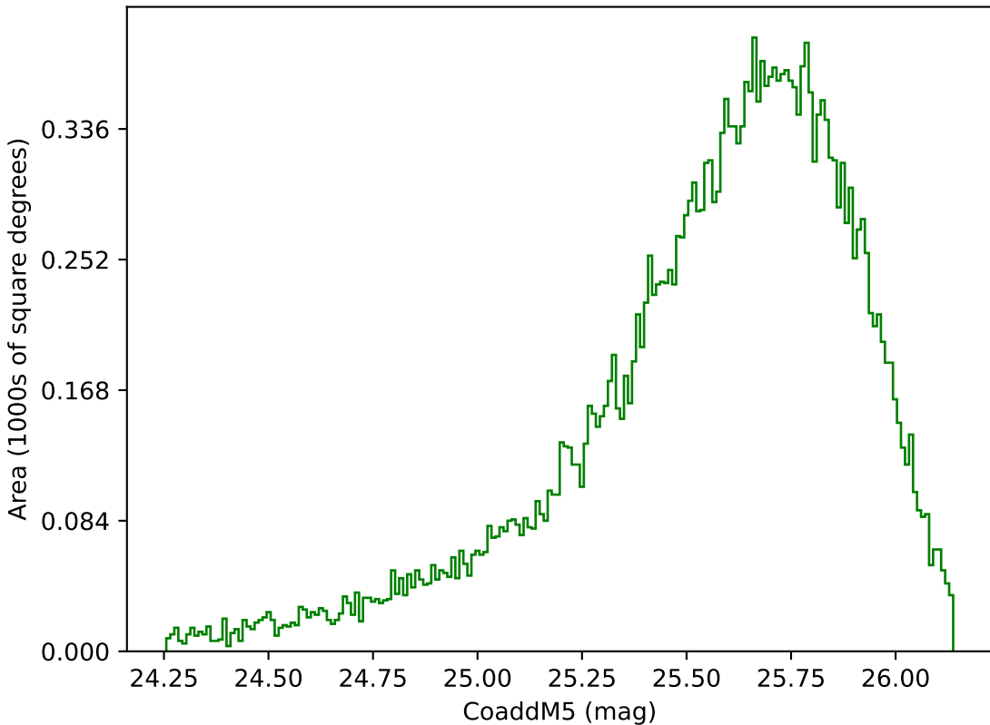
too_10_4v3.4_10yrs Yr 1 g band: CoaddM5
