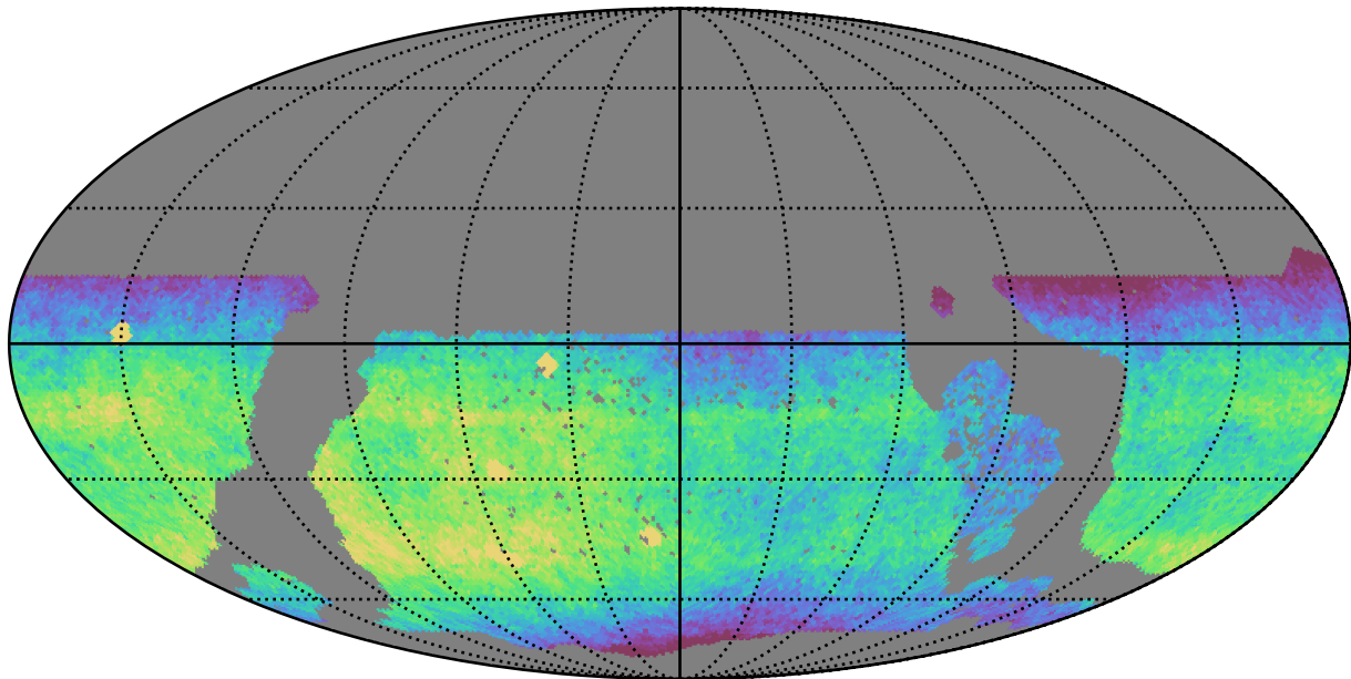
too_10_4v3.4_10yrs WFD z band: CoaddM5
