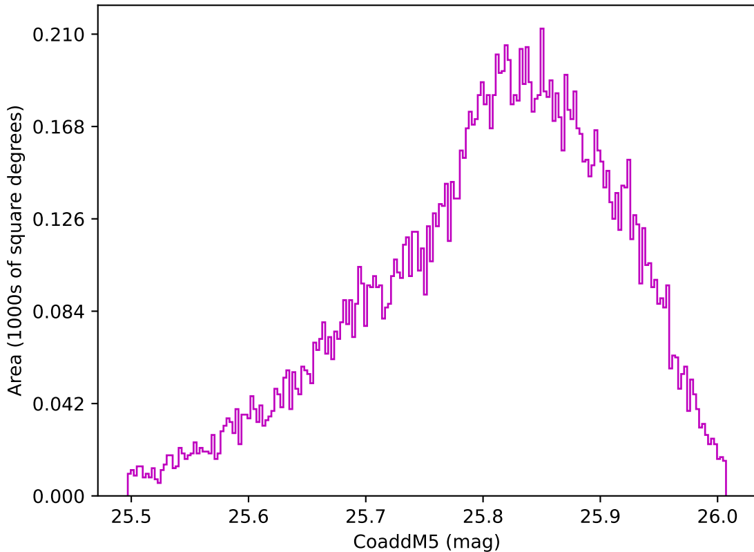
too_10_4v3.4_10yrs WFD z band: CoaddM5
