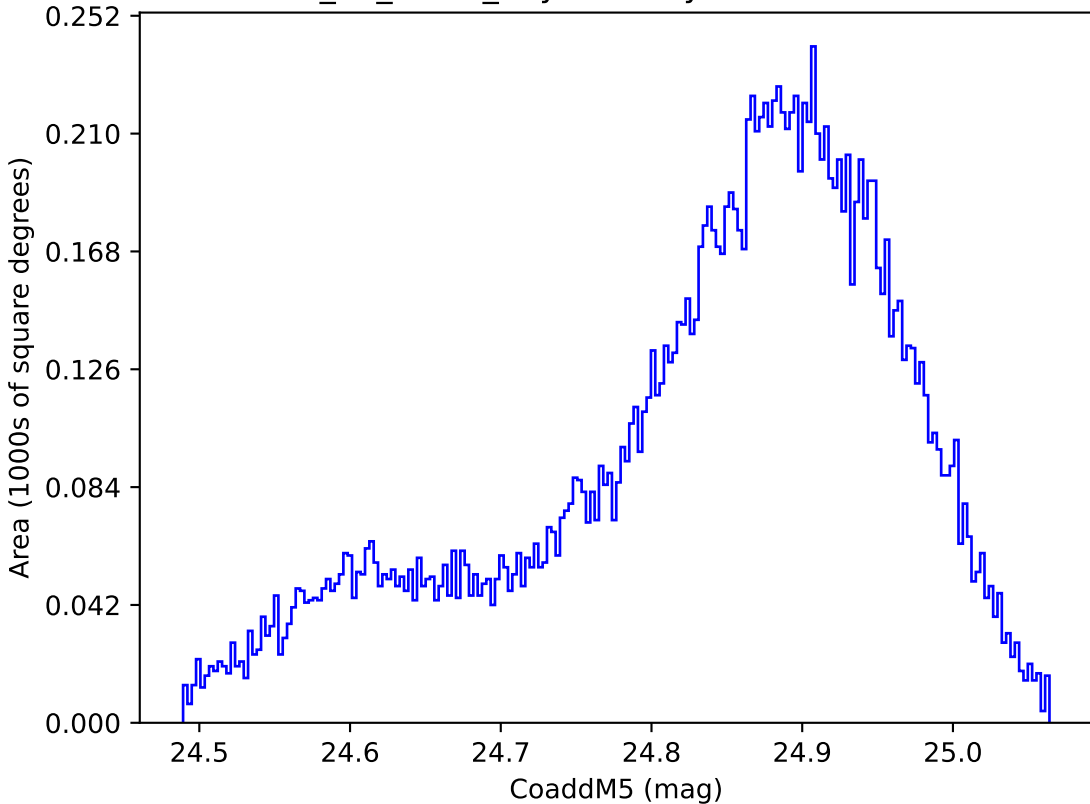
too_10_4v3.4_10yrs WFD y band: CoaddM5
