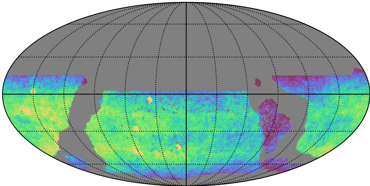
too_10_4v3.4_10yrs WFD u band: CoaddM5
