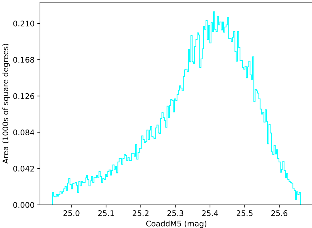
too_10_4v3.4_10yrs WFD u band: CoaddM5
