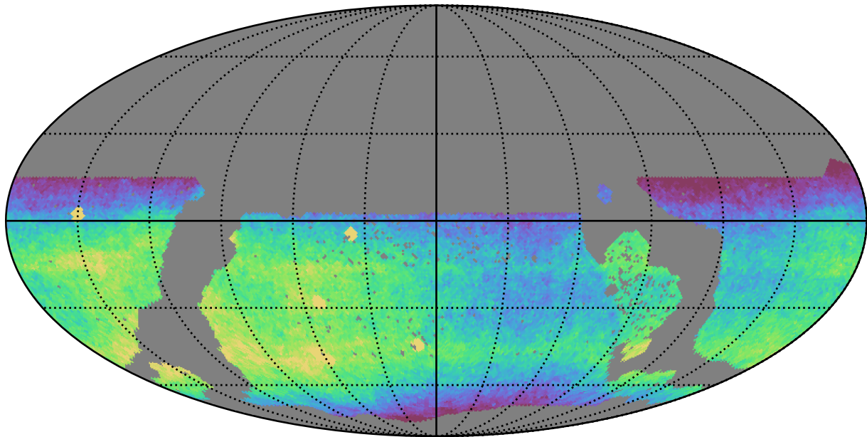
too_10_4v3.4_10yrs WFD r band: CoaddM5
