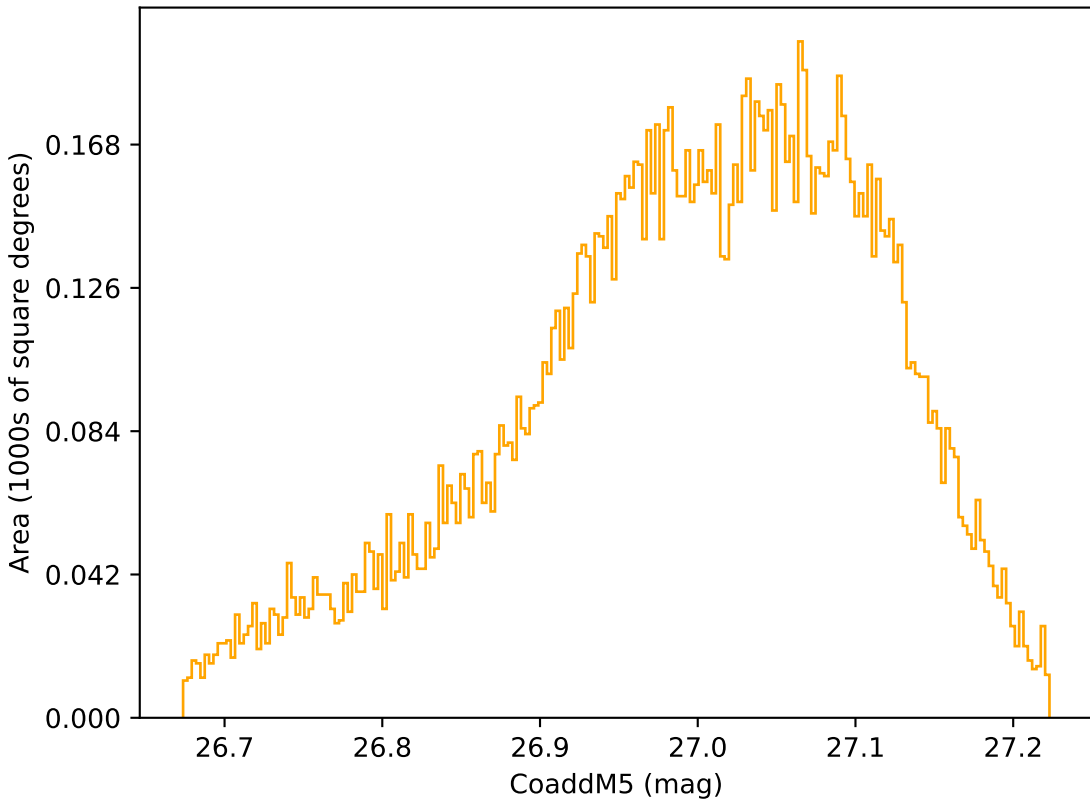
too_10_4v3.4_10yrs WFD r band: CoaddM5
