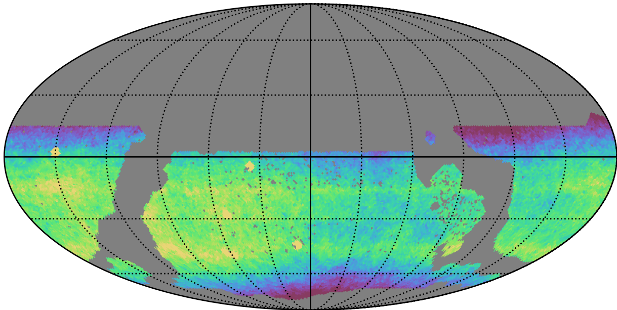
too_10_4v3.4_10yrs WFD i band: CoaddM5
