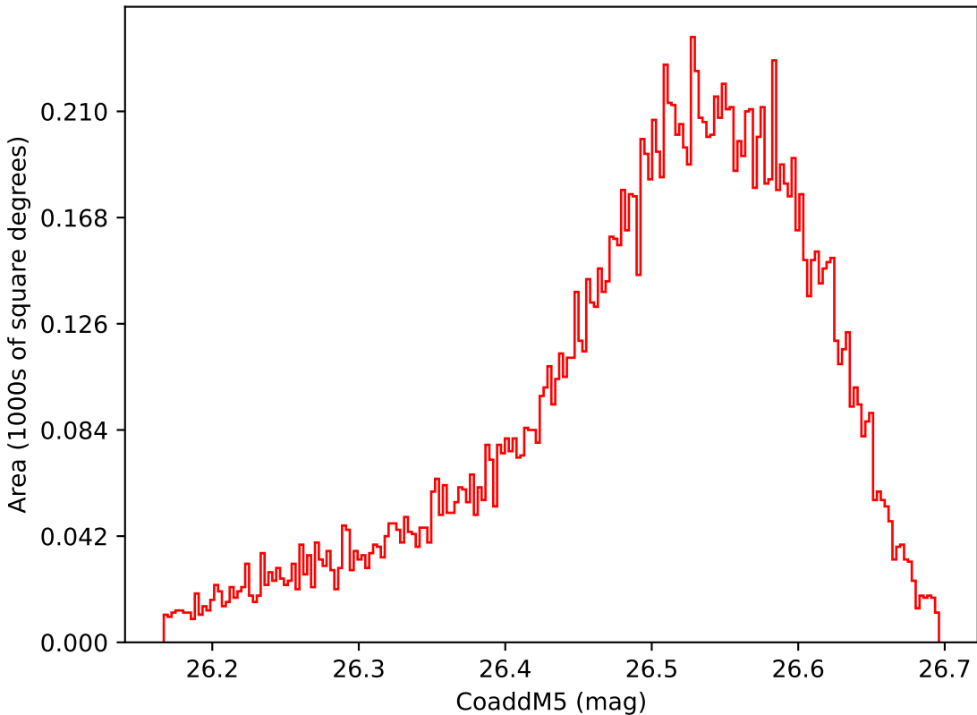
too_10_4v3.4_10yrs WFD i band: CoaddM5
