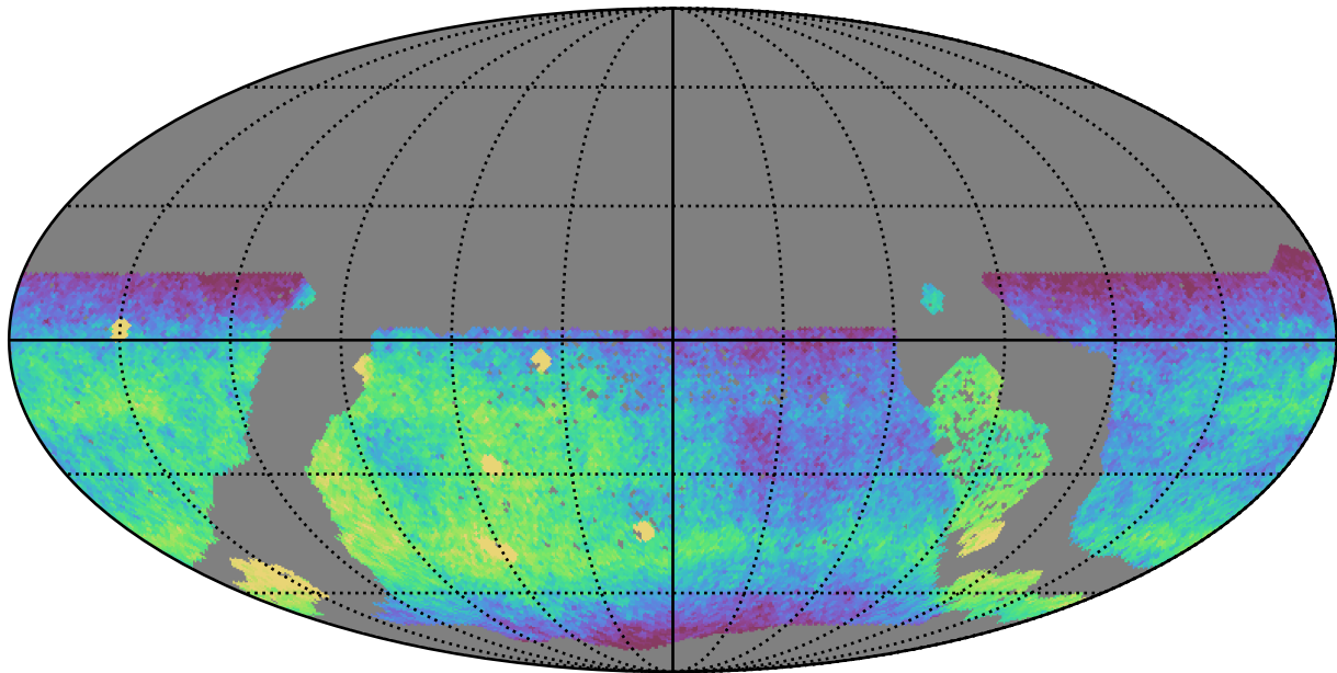
too_10_4v3.4_10yrs WFD g band: CoaddM5
