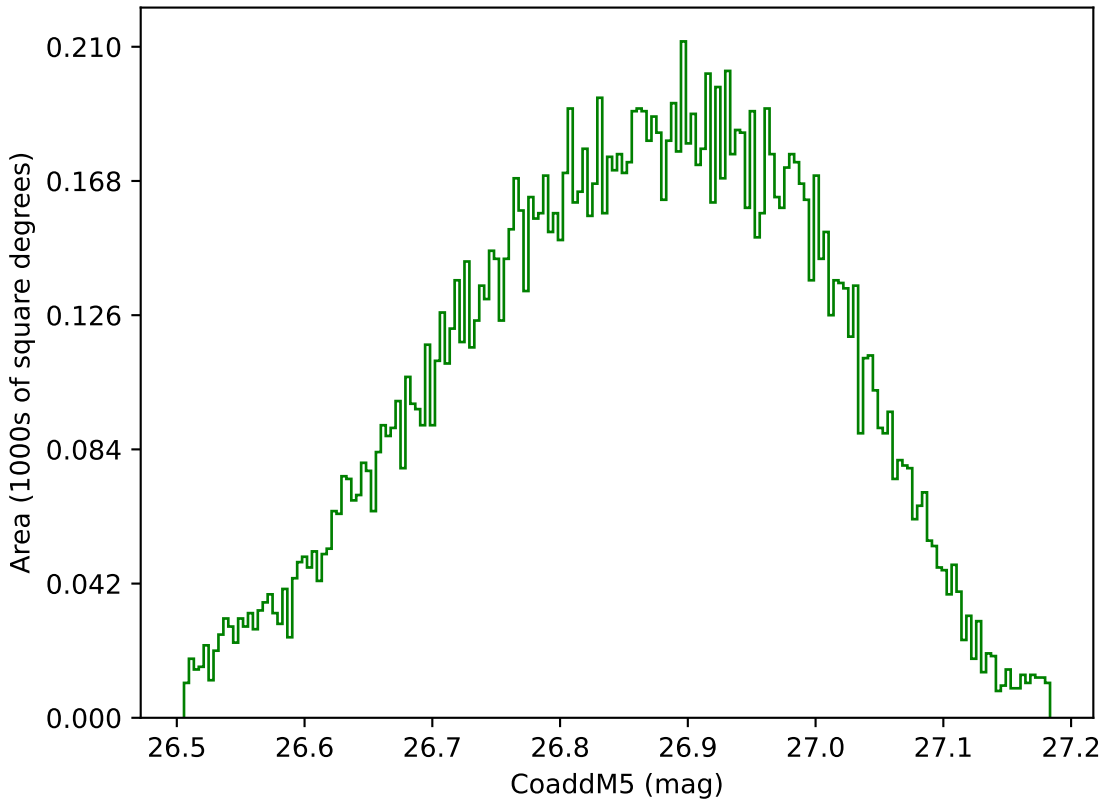
too_10_4v3.4_10yrs WFD g band: CoaddM5
