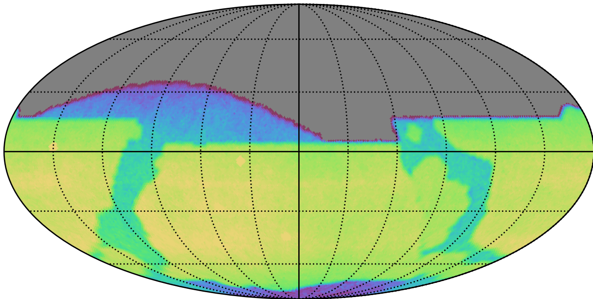
too_10_4v3.4_10yrs All sky z band: CoaddM5
