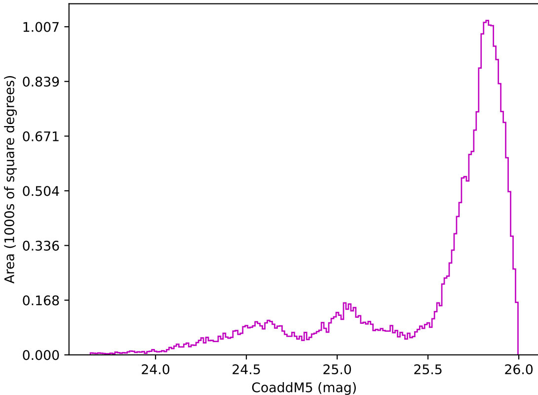
too_10_4v3.4_10yrs All sky z band: CoaddM5
