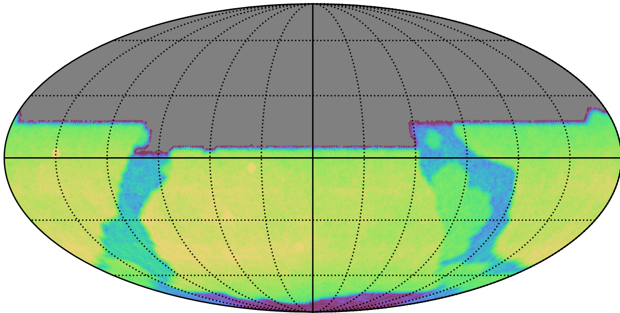
too_10_4v3.4_10yrs All sky y band: CoaddM5
