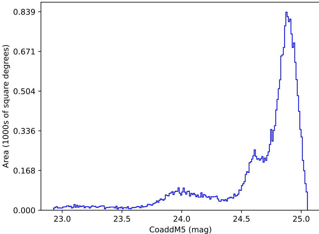
too_10_4v3.4_10yrs All sky y band: CoaddM5
