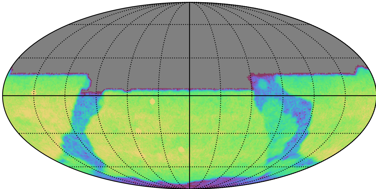
too_10_4v3.4_10yrs All sky u band: CoaddM5
