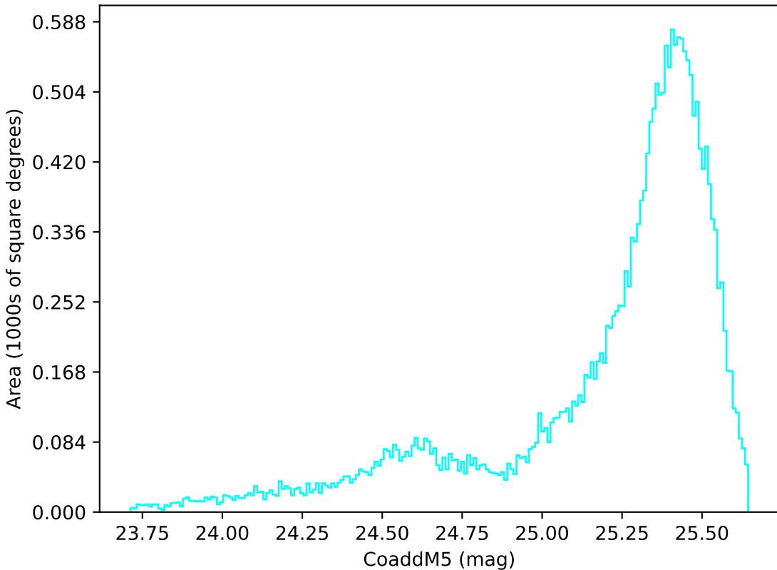
too_10_4v3.4_10yrs All sky u band: CoaddM5
