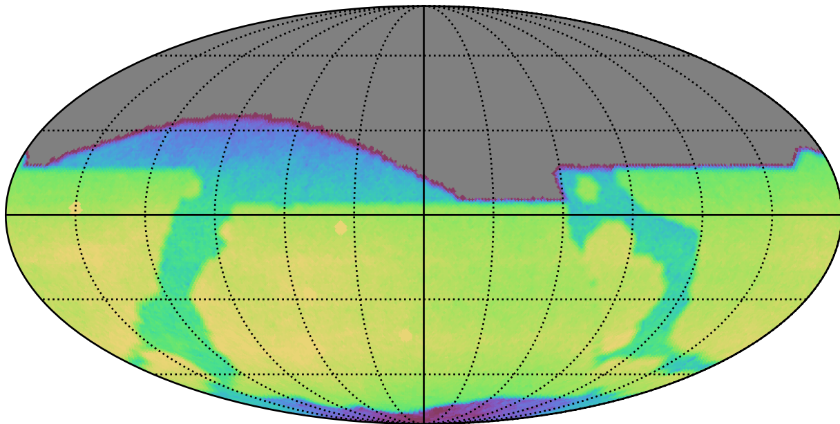
too_10_4v3.4_10yrs All sky r band: CoaddM5
