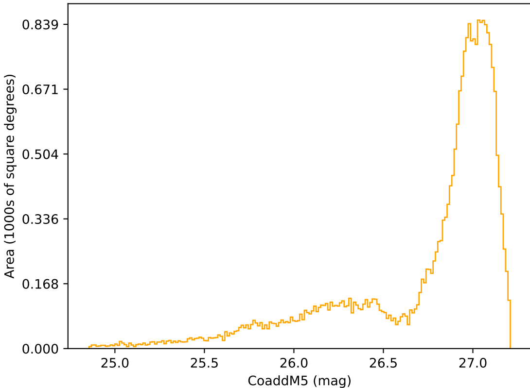
too_10_4v3.4_10yrs All sky r band: CoaddM5
