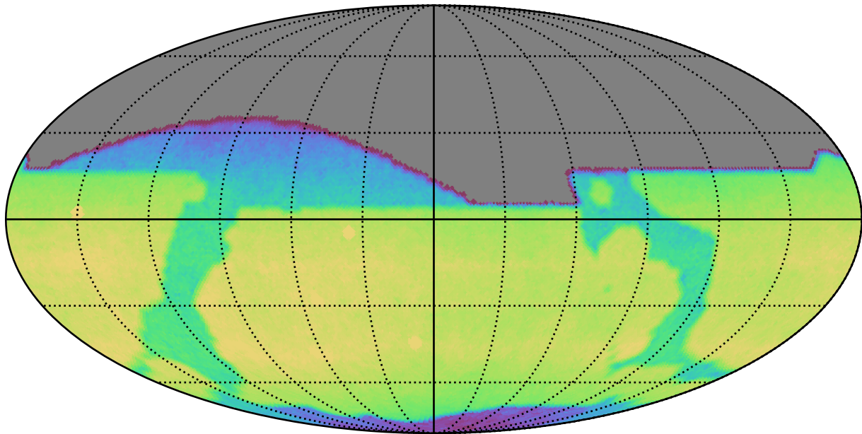
too_10_4v3.4_10yrs All sky i band: CoaddM5
