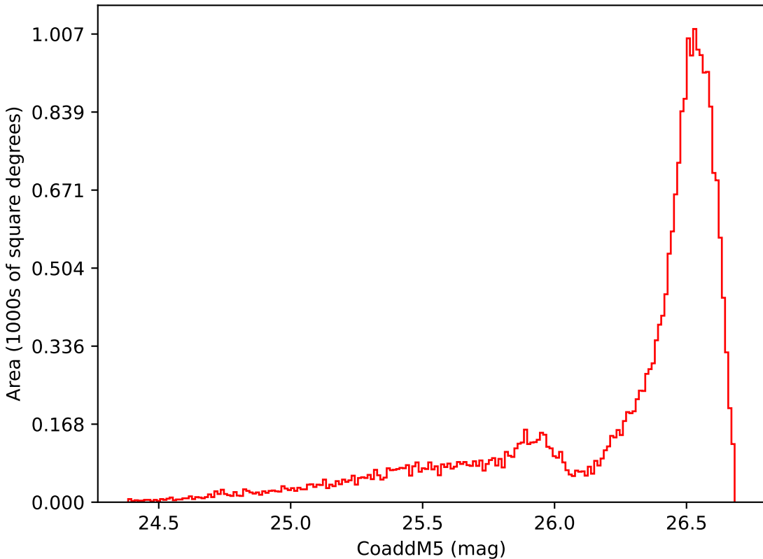
too_10_4v3.4_10yrs All sky i band: CoaddM5
