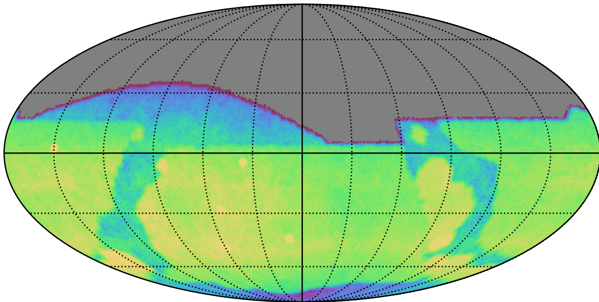
too_10_4v3.4_10yrs All sky g band: CoaddM5
