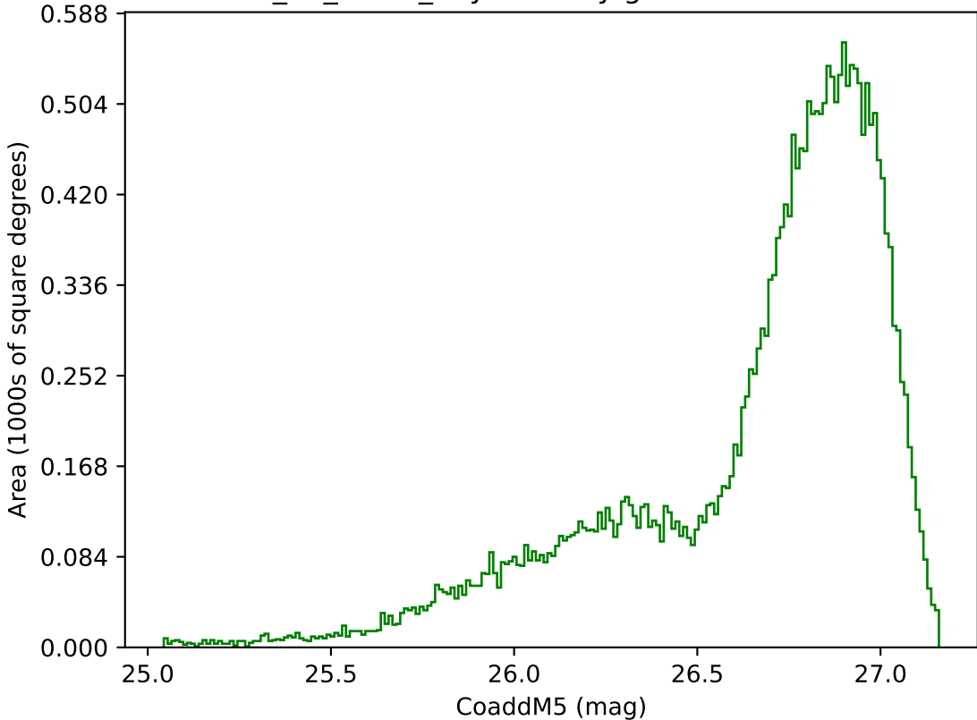
too_10_4v3.4_10yrs All sky g band: CoaddM5
