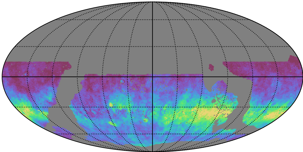
too_10_4v3.4_10yrs WFD z band: AngleRms rotSkyPos
