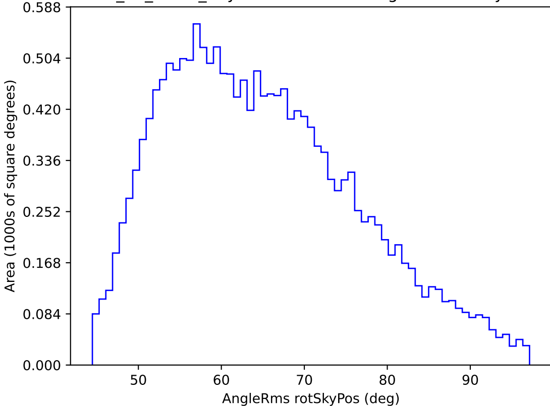
too_10_4v3.4_10yrs WFD u band: AngleRms rotSkyPos
